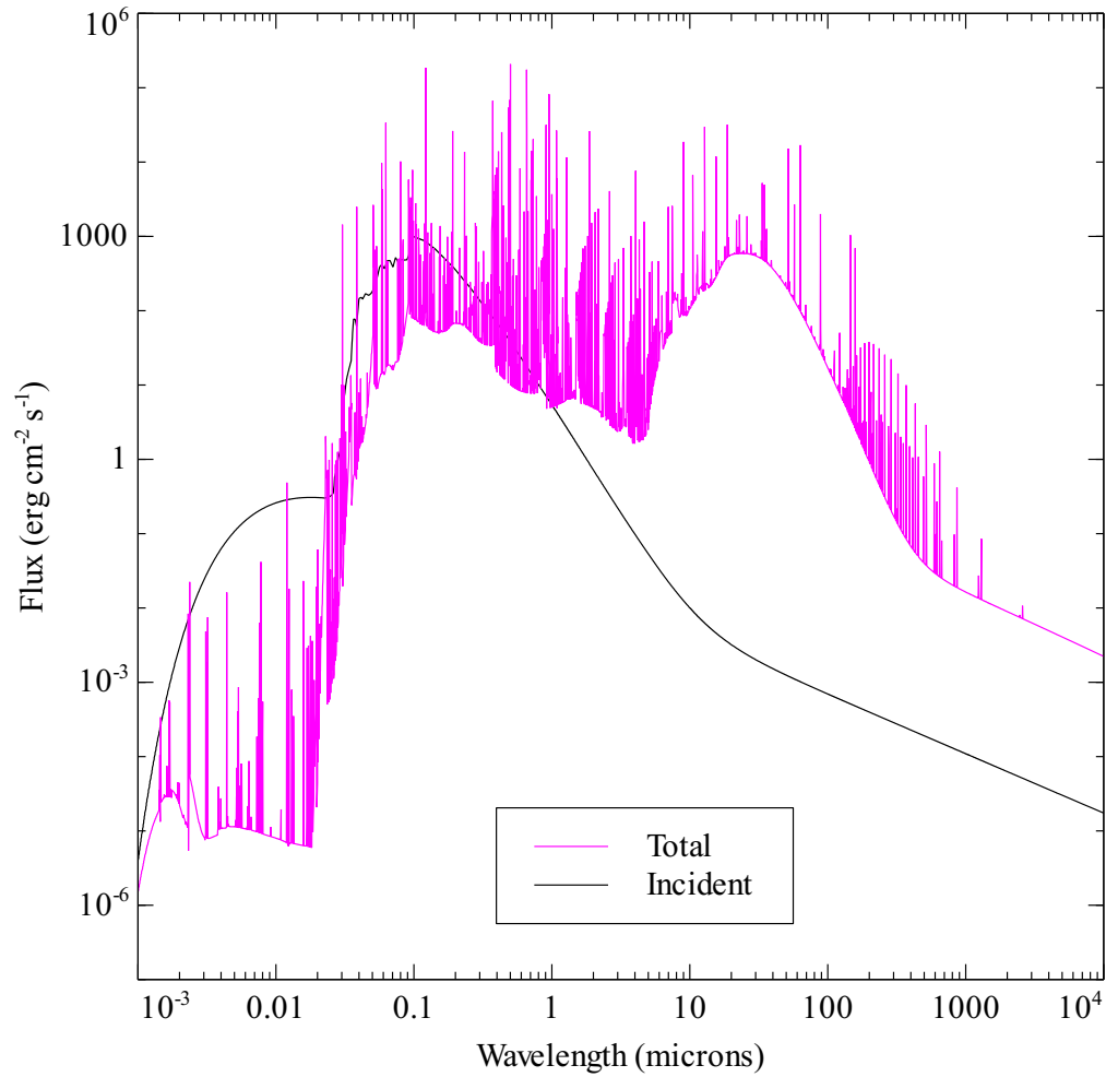
Figure 5: The incident (smooth) and emitted spectrum contained in the orion_hii_pdr_pp.con file. The x-axis is the wavelength in microns and the y-axis gives \nu f_\nu [erg cm -2 s -1 ]. This is produced by the save continuum command.
