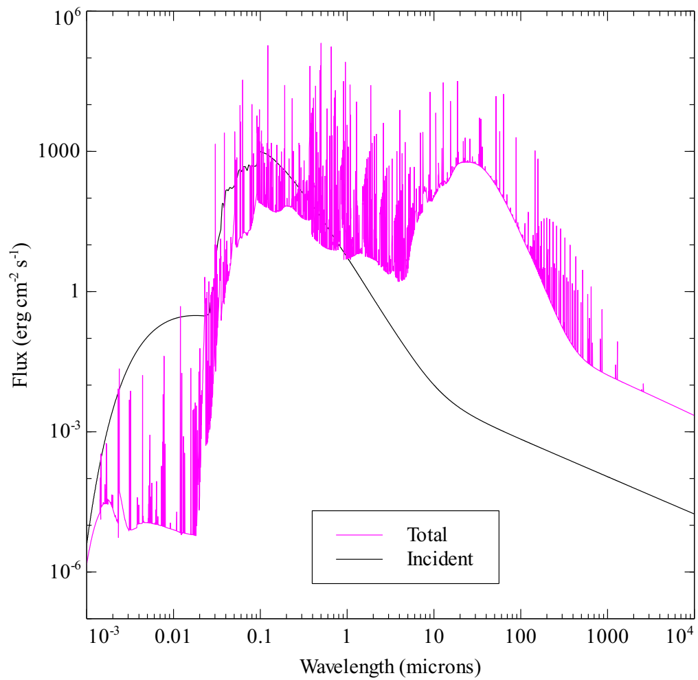
Figure 5: The incident (smooth) and emitted spectrum contained in the orion_hii_pdr_pp.con file. The x-axis is the wavelength in micron and the y-axis gives \nu f_\nu [ \text{erg cm}^{-2} \text{s}^{-1} ]. This is produced by the save continuum command.
